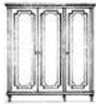
8300 3 DOORS WARDROBE 150 x 64 x 230 h
